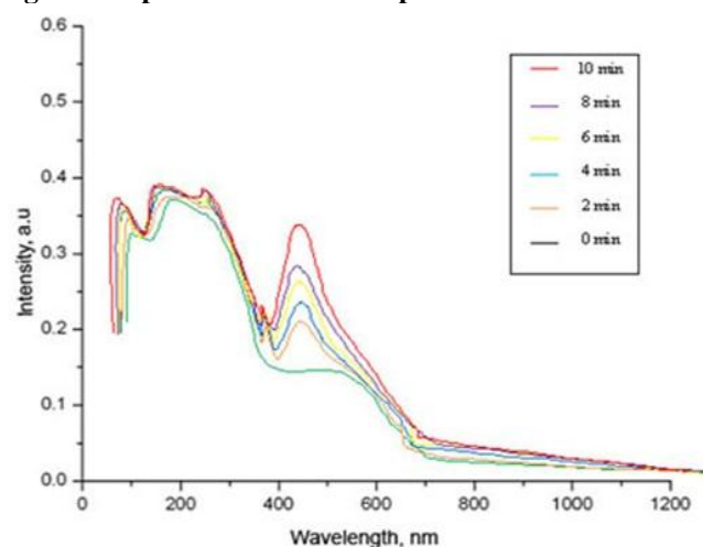
Fig 2. UV Spectra of silver nanoparticles
