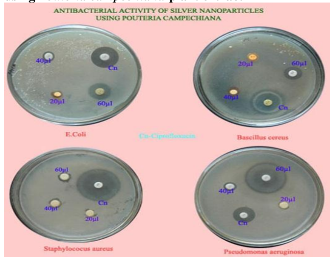
Fig 6. Antibacterial activity of silver Nanoparticles using Pouteria campechiana plant extract
