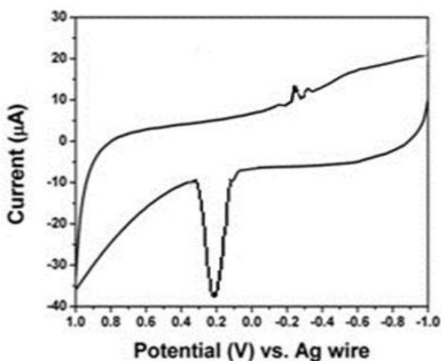
Fig 5. Cyclic voltammograms of silver nanoparticles
